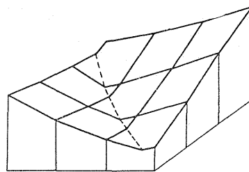
Figure 2: Grid DTM with a break line
