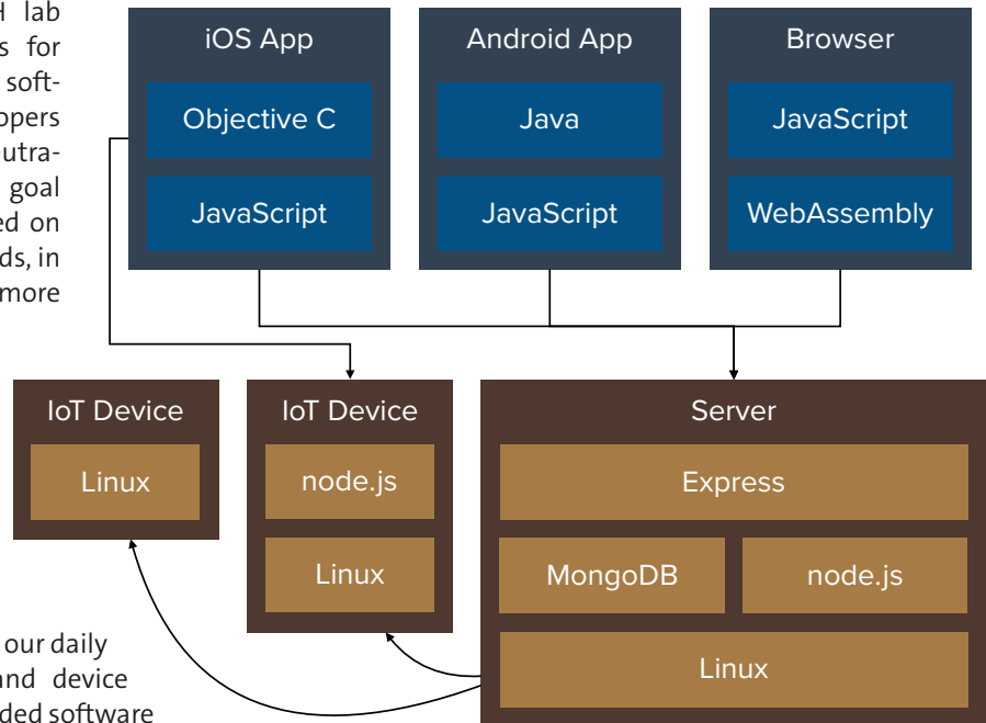
Modern system stacks combine many different programming languages and platforms.
