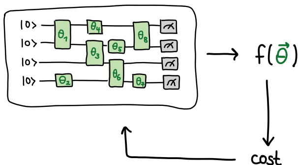
Visualization of a circuit for quantum variational algorithms.
